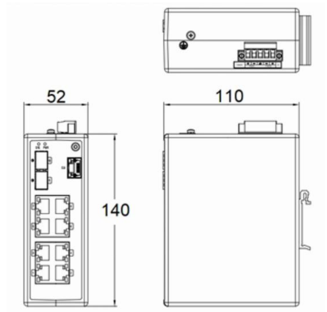
ISM5010D Dimensional diagram
