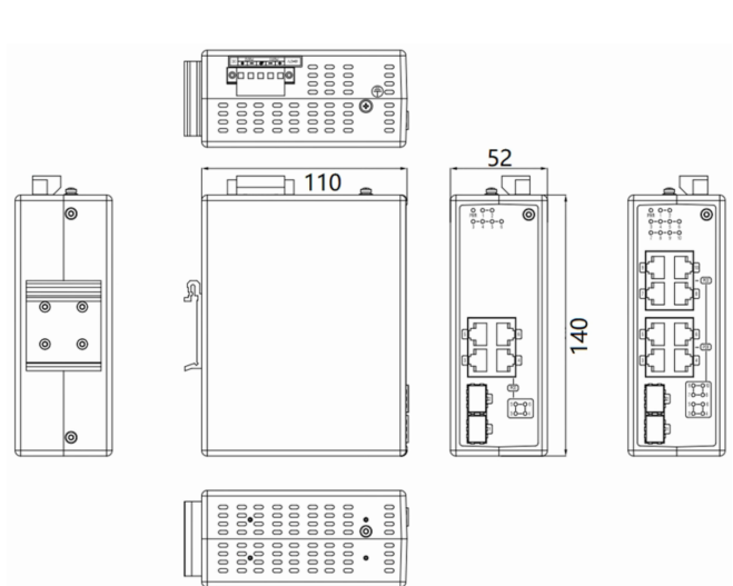
ISE5310D Dimensional diagram
