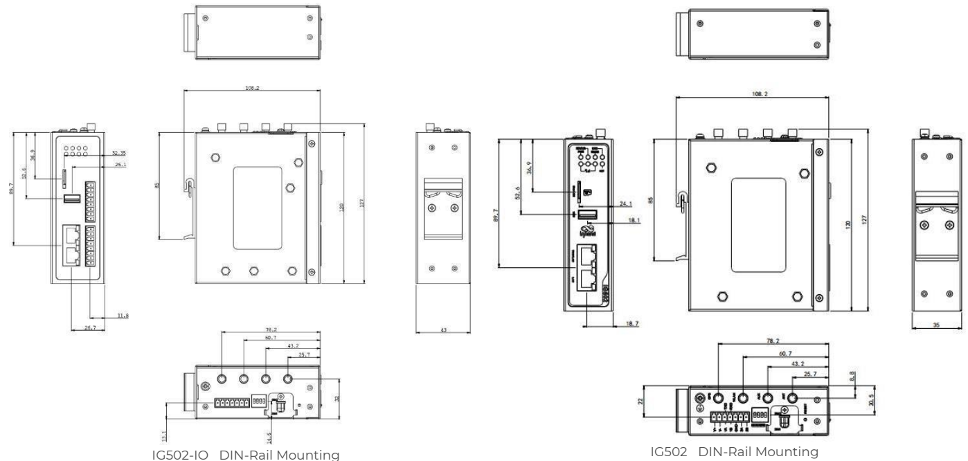
IG502-IO DIN-Rail Mounting
